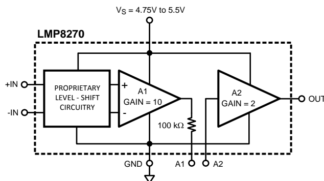
Figure 21. LMP8270
