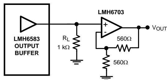
Figure 38. Buffered Output
