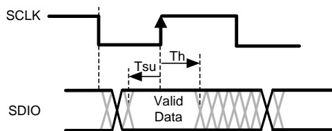
Figure 67. Write Timing
