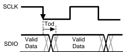
Figure 66. Read Timing
