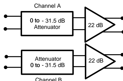
Figure 42. LMH6517 Block Diagram
