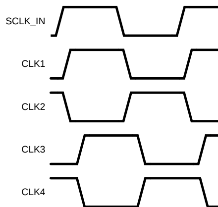
Figure 22. Clock Outputs Timing: With Skew and Inversion
