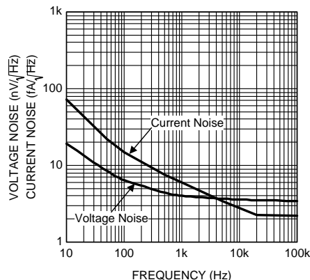
Figure 1. Current Noise and Voltage Spectral Density
