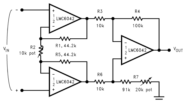
Figure 41. Instrumentation Amplifier
