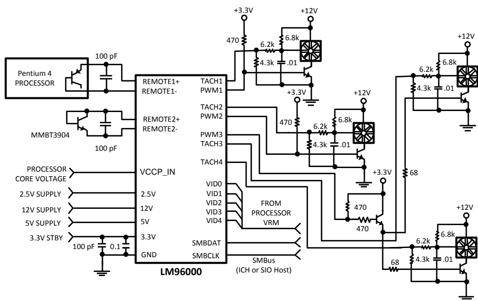
Figure 11. Typical Applications Schematic
