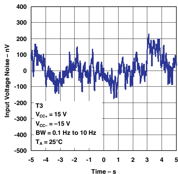
LOW-FREQUENCY NOISE
