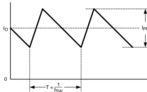
Figure 7. Inductor Current
