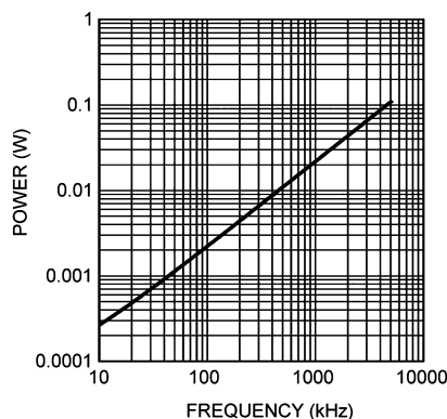
Figure 19. Forward Bias Power Loss of Bootstrap Diode V_{\text{IN}}=50\text{V}
