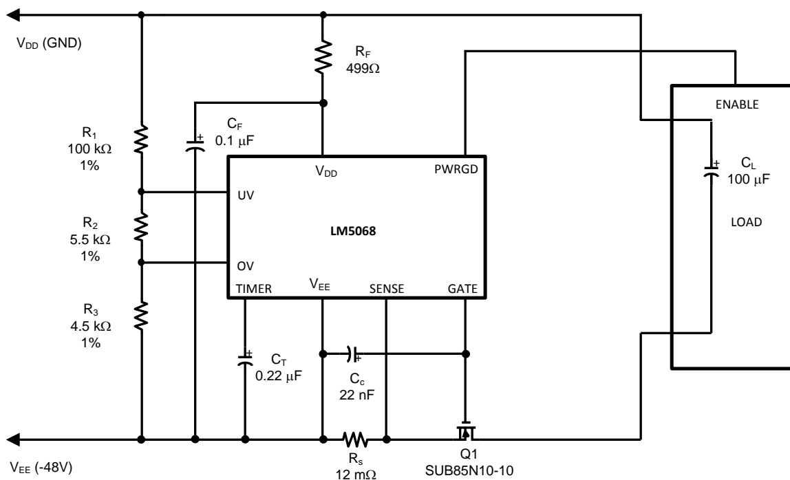
Figure 1. Negative Power Supply Control
