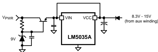
Figure 19. Start-up Regulator for V_{PWR} > 100V
