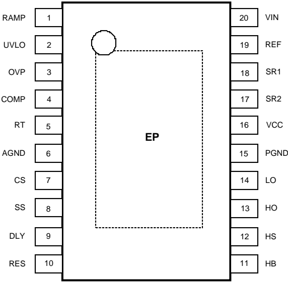
Figure 1. LM5035A 20-Lead HTSSOP (Top View )
