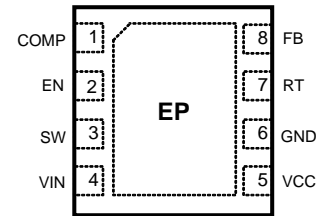
Figure 3. Top View WSON-8 Package
