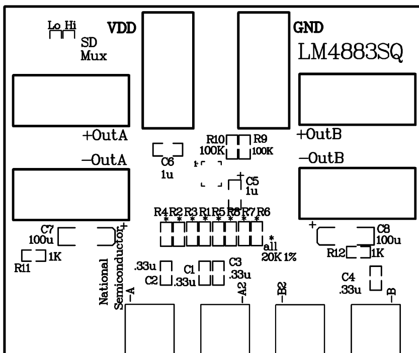
Figure 48. Silkscreen
