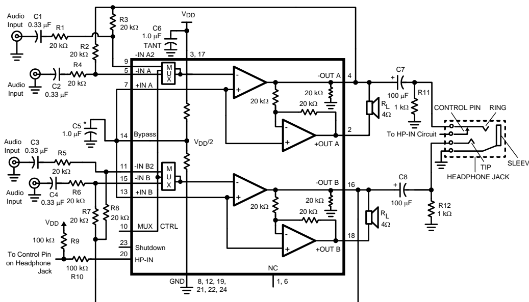
Figure 44. Typical Audio Amplifier Application Circuit
