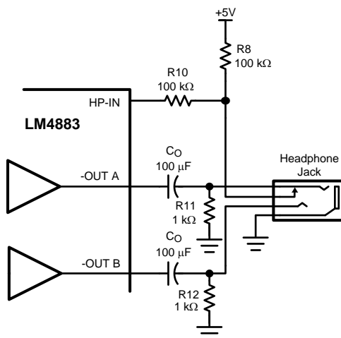
Figure 45. Headphone Circuit
