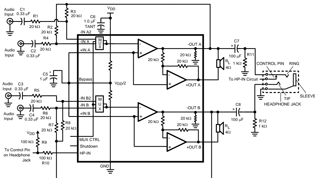
Figure 2. Typical Audio Amplifier Application Circuit
