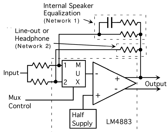
Figure 43. Input MUX Example
