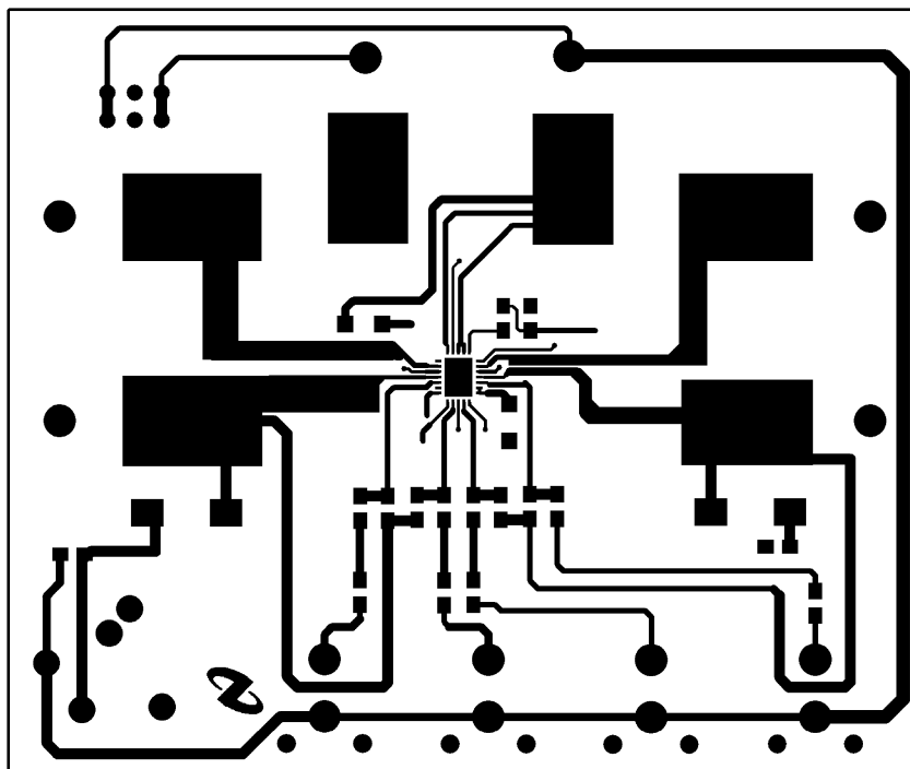
Figure 46. Top Layer
