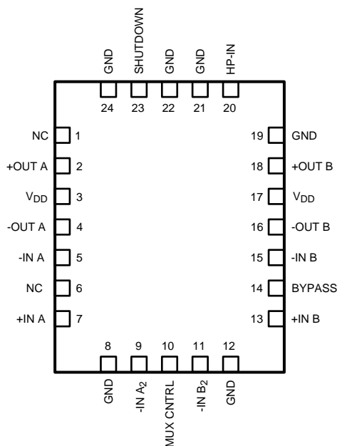
Figure 1. LM4883SQ Top View See Package Number NHZ0024B
