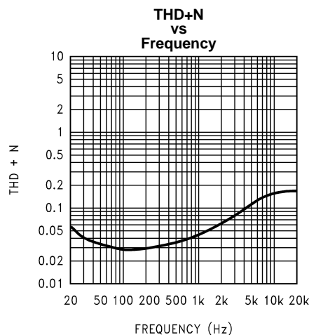
Figure 9. V_{DD} = 3V ; LLS, RLS; P_O = 200mW ; R_L = 8\Omega ; Mode 7; 0dB Gain
