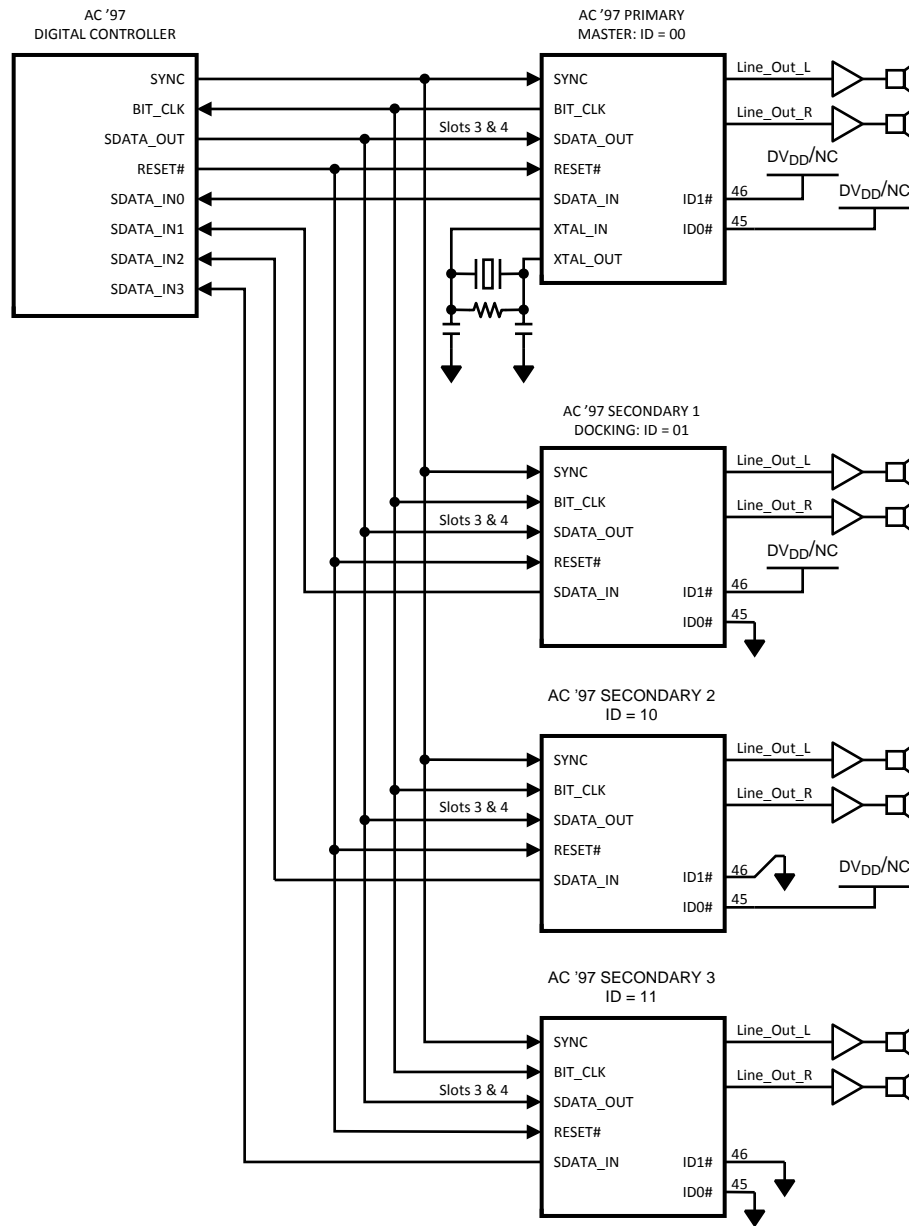
Figure 23. Multiple Codecs using Extended AC Link
