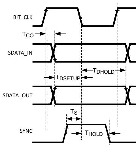
Figure 2. Data Delay, Setup and Hold
