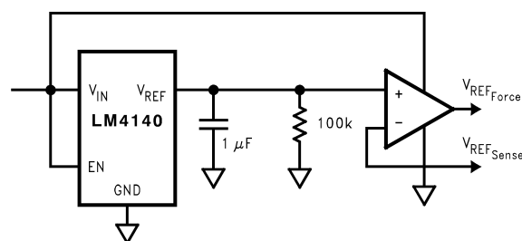
Figure 32. Voltage Reference with Force and Sense Output
