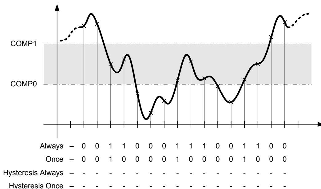
Figure 13-16. Mid-Band Operation (CIC=0x1)
