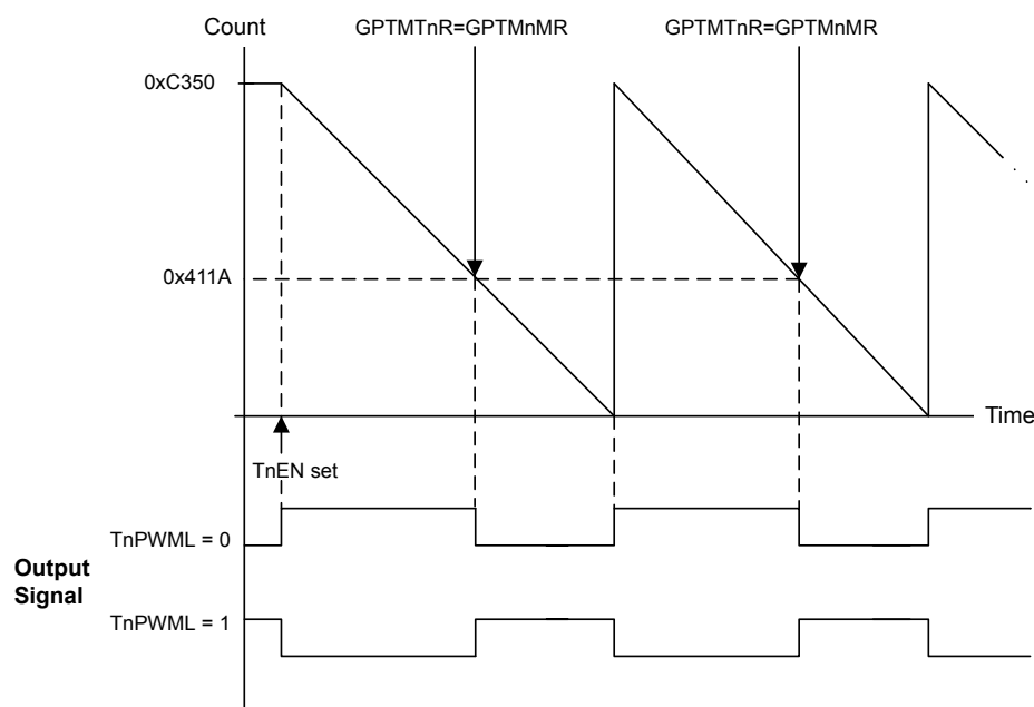
Figure 9-5. 16-Bit PWM Mode Example
