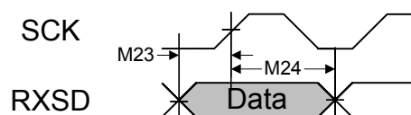
Figure 25-19. I 2 S Slave Mode Receive Timing
