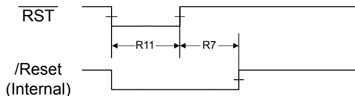
Figure 23-6. Power-On Reset Timing
