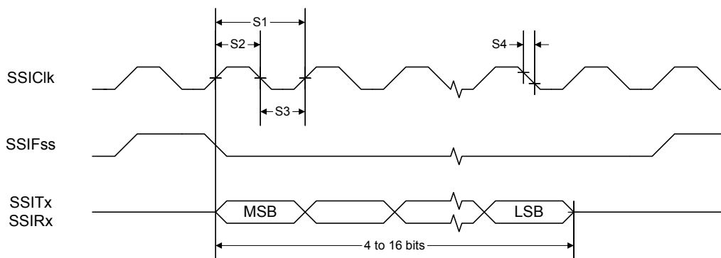
Figure 21-11. SSI Timing for TI Frame Format (FRF=01), Single Transfer Timing Measurement
