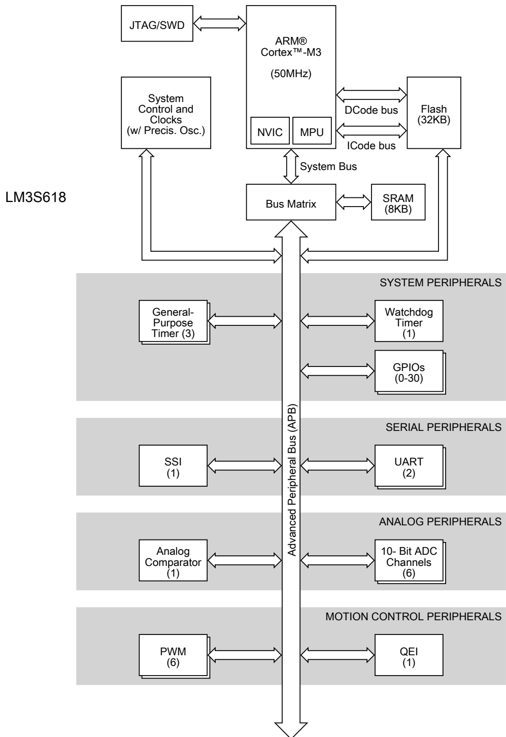
Figure 1-1. Stellaris LM3S618 Microcontroller High-Level Block Diagram
