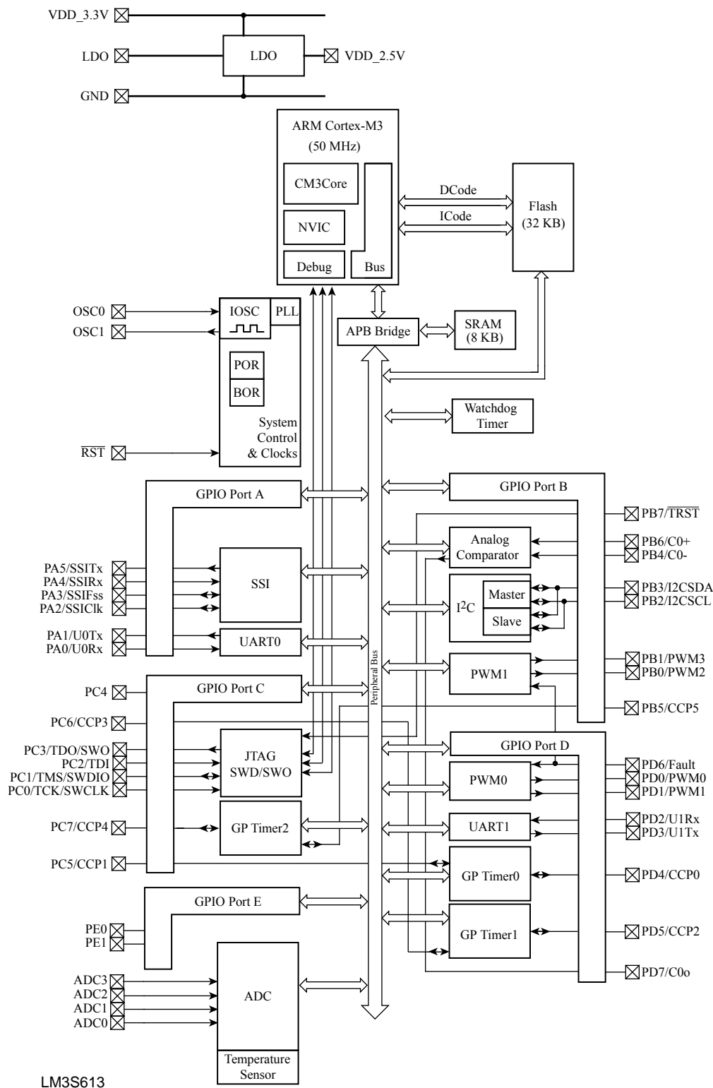
Figure 1-2. LM3S613 Controller System-Level Block Diagram
