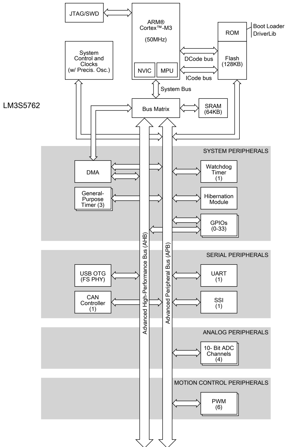
Figure 1-1. Stellaris LM3S5762 Microcontroller High-Level Block Diagram
