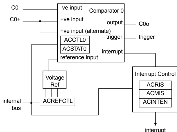
Figure 16-1. Analog Comparator Module Block Diagram
