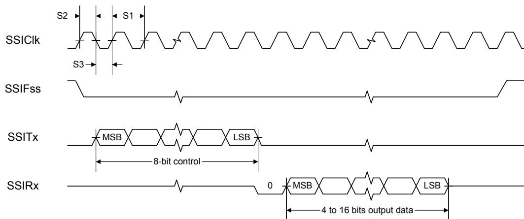
Figure 21-11. SSI Timing for MICROWIRE Frame Format (FRF=10), Single Transfer
