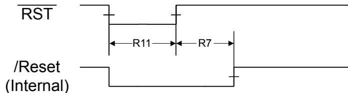
Figure 22-5. Power-On Reset Timing
