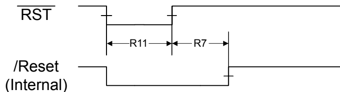
Figure 20-5. Power-On Reset Timing
