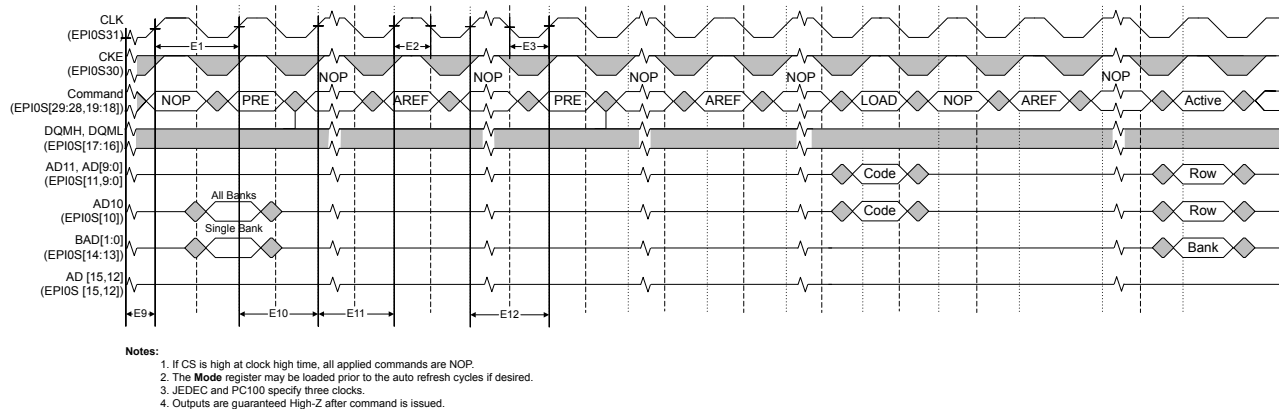
Figure 21-13. SDRAM Initialization and Load Mode Register Timing
