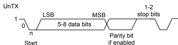
Figure 11-2. UART Character Frame
