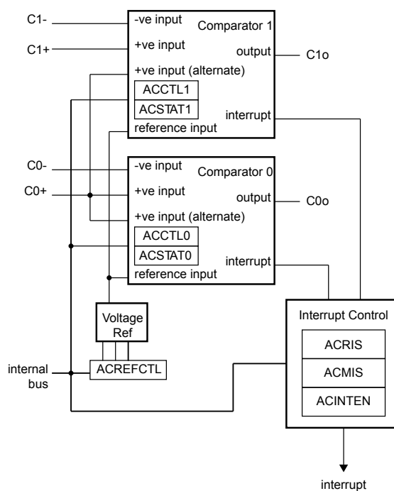
Figure 13-1. Analog Comparator Module Block Diagram
