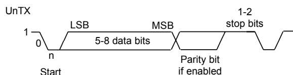
Figure 10-2. UART Character Frame
