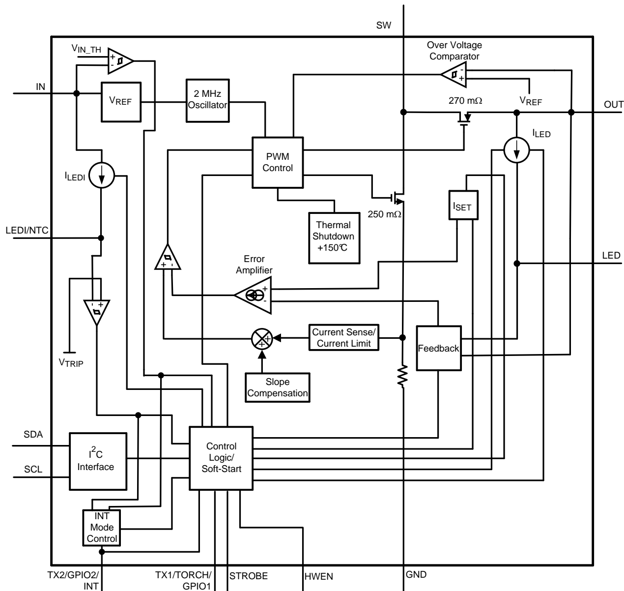
Figure 24. Block Diagram
