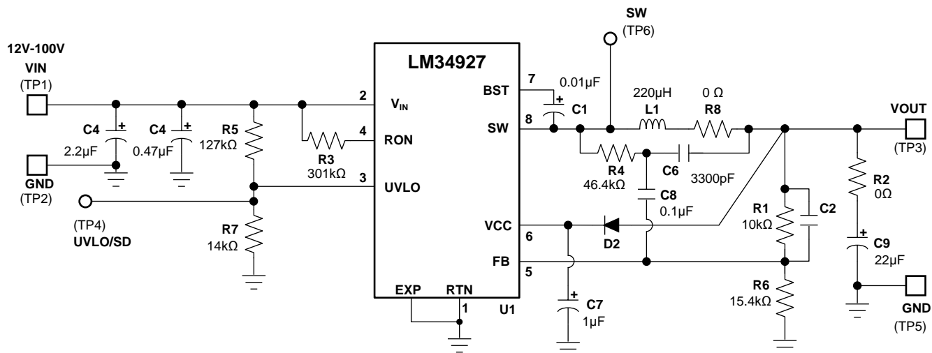
Figure 21. TYPICAL BUCK CONFIGURATION: V in = 9V to 100V, V out = 3.3V, I out = 500mA
