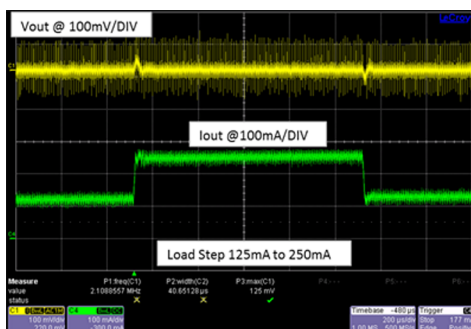
Figure 27. Buck Transient Response 72Vin
