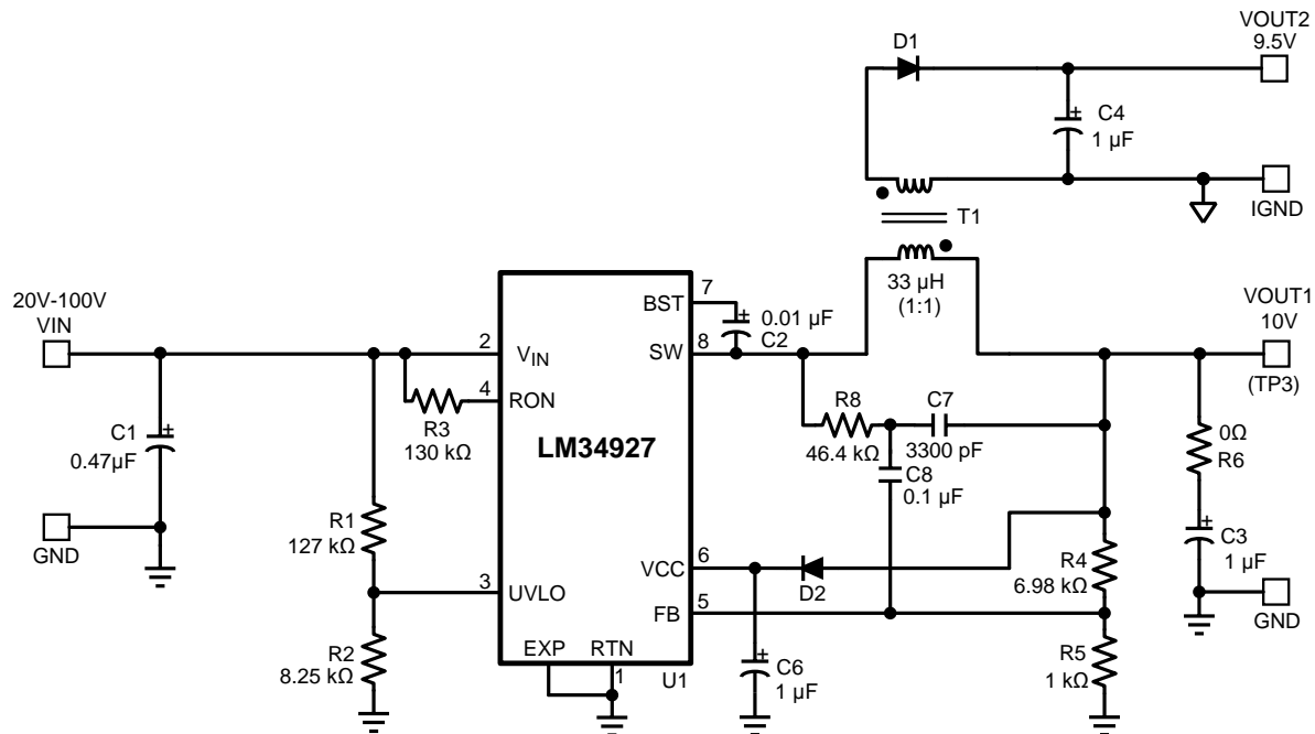
Figure 17. A 3W Isolated Application Schematic
