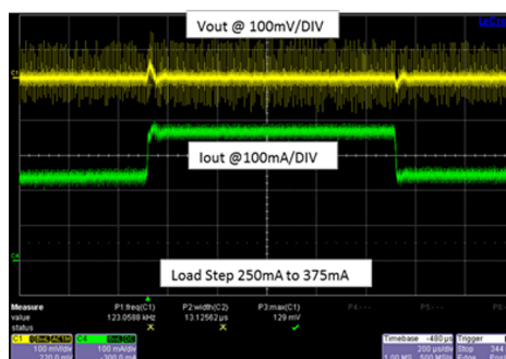
Figure 26. Buck Transient Response 48Vin
