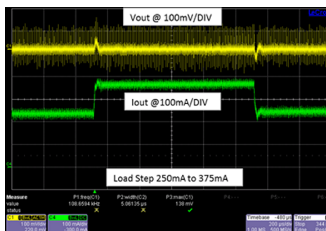
Figure 28. Buck Transient Response 72Vin
