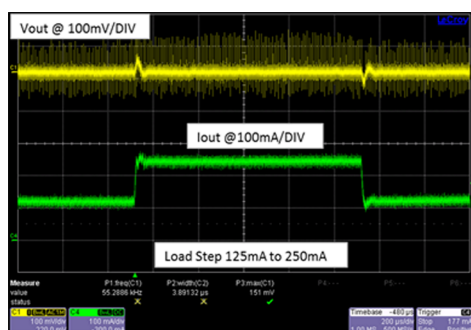
Figure 23. Buck Transient Response 36Vin
