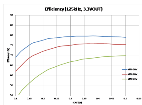
Figure 22. Efficiency
