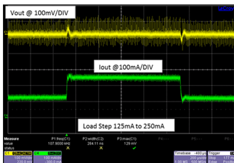
Figure 25. Buck Transient Response 48Vin
