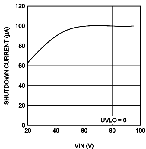
Figure 11. I_{IN} vs V_{IN} (Shutdown)
