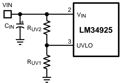
Figure 15. UVLO Resistor Setting
