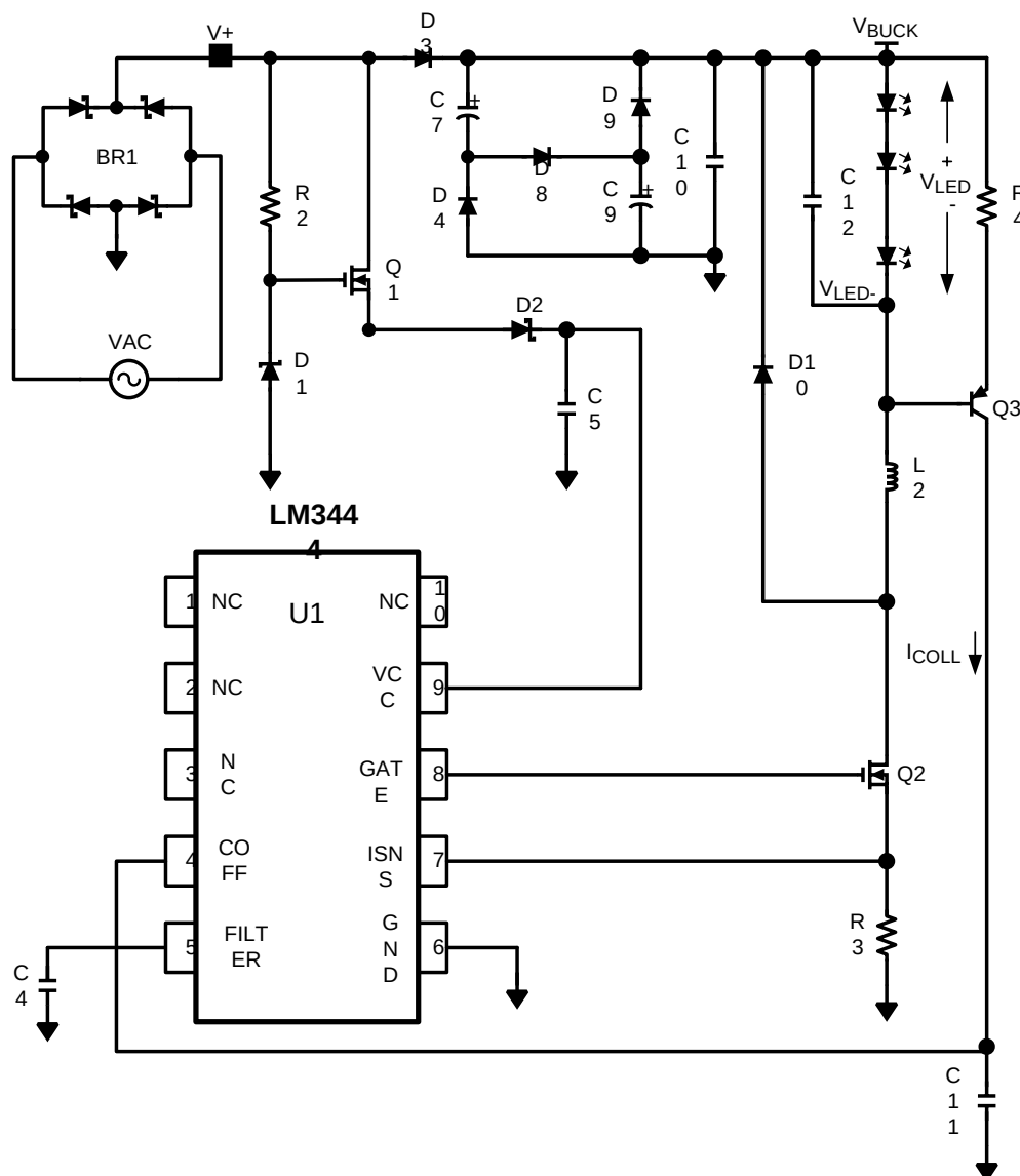
Figure 11. LM3444 Schematic
