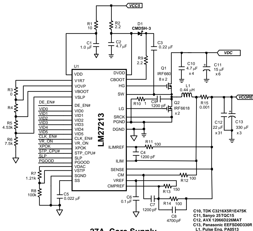
27A Core Supply
