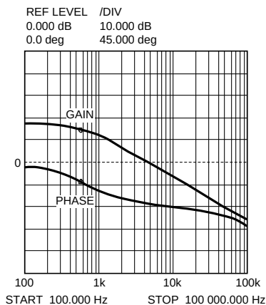
Figure 16. Gain and Phase of Modulator R_{\text{LOAD}} = 20\text{ Ohms} and C_{\text{OUT}} = 22\mu\text{F}
