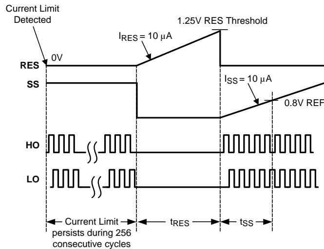
Figure 27. Hiccup Mode Current Limit Timing Diagram
