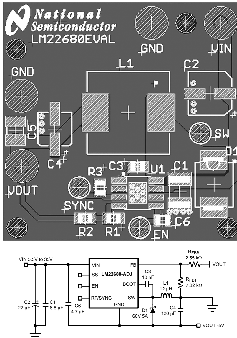
Figure 24. Inverting Regulator Application
