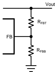
Figure 16. Resistive Feedback Divider
