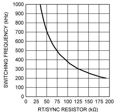
Figure 17. Switching Frequency vs RT/SYNC Resistor
