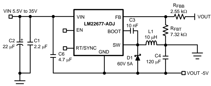
Figure 23. Inverting Regulator Application
