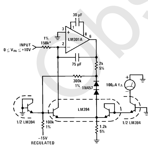
Low Cost Accurate Square Root Circuit I_{OUT} = 10^{-5} \cdot \sqrt{10 V_{IN}}
