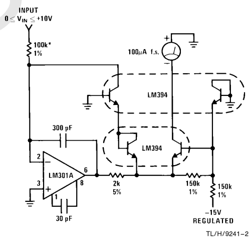
Low Cost Accurate Squaring Circuit I_{OUT} = 10^{-6} (V_{IN})^2
