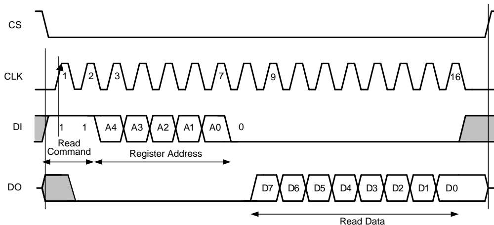
Figure 23. SPI Interface Read
