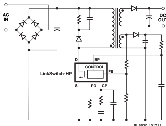
Figure 1. Typical Application Schematic.
