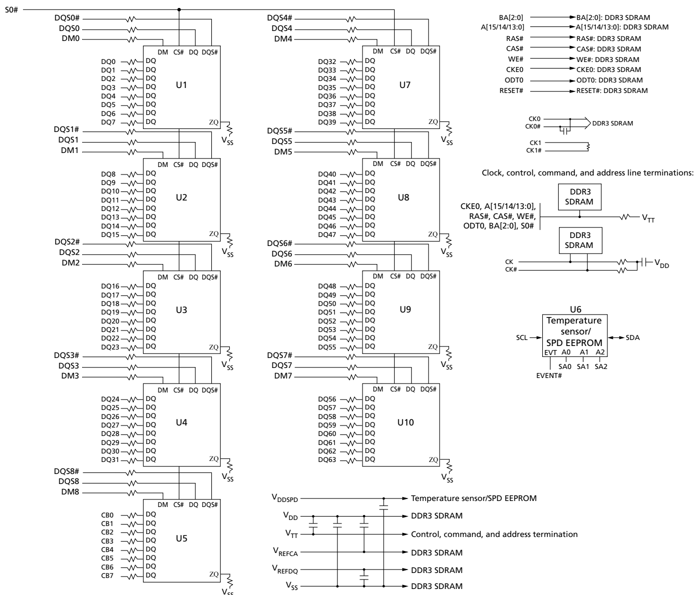
Figure 4: Functional Block Diagram (PCB 1483)
