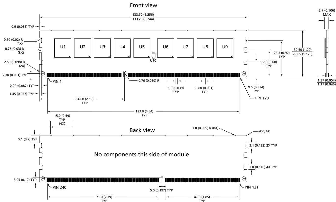
Figure 5: 240-Pin DDR3 UDIMM – PCB 1125
