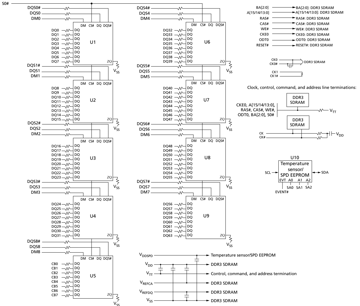
Figure 3: Functional Block Diagram (PCB 1125)
