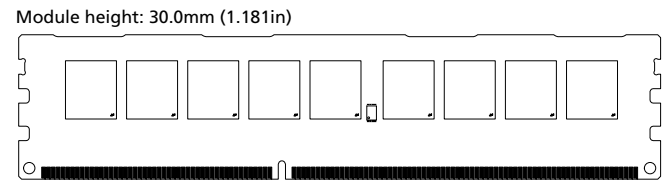
Figure 2: 240-Pin UDIMM (MO-269 R/C D1) PCB 1483
