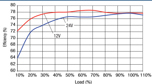
NCS6D1215C
