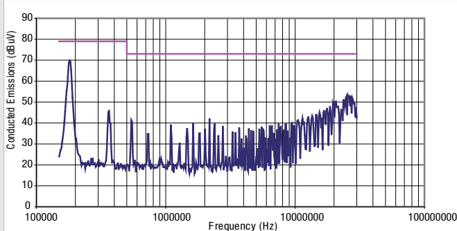
NCS6S1215C
