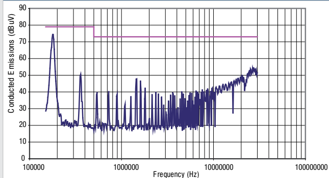
NCS6S4812C
