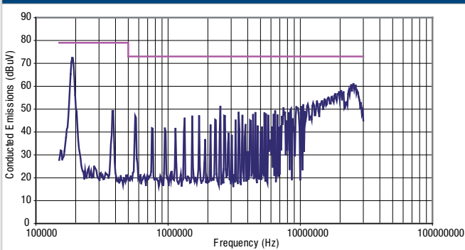
NCS6D4805C
