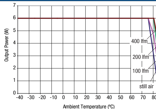
NCS6S4815C
