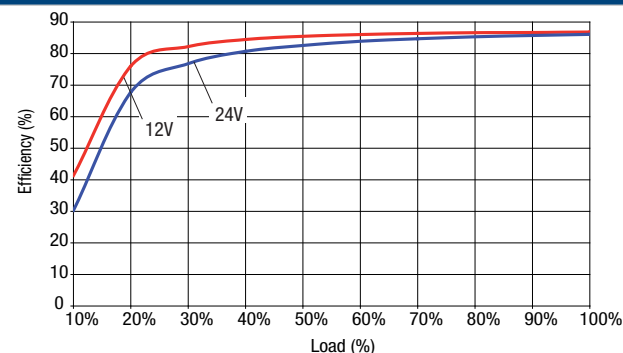
NCS6S4805C
