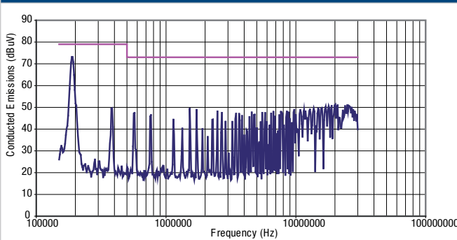
NCS6D4812C
