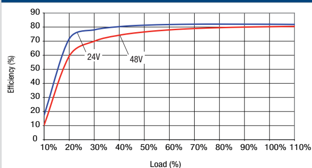
NCS6S4805C
