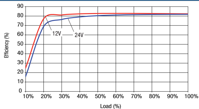
NCS6S1215C
