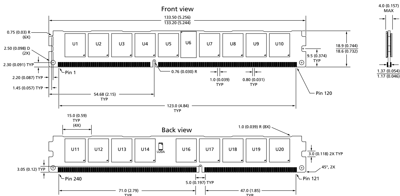
Figure 3: 240-Pin DDR3 VLP RDIMM
