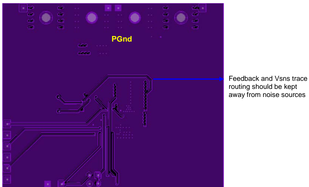
Figure 44: IRDC3827 Demo Board – Middle Layer 2
