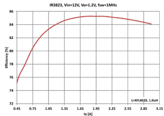
Figure 2: IR3823 Efficiency
